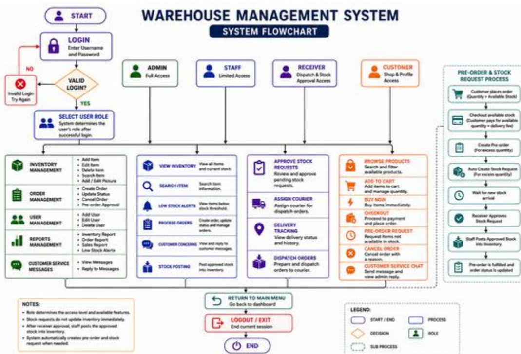
Figure 10: Warehouse Management System Flowchart
